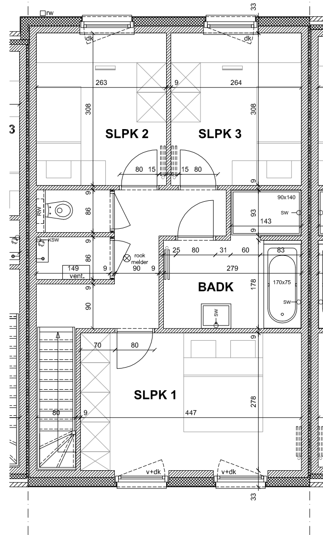
VERDIEPING OPP. 53,58 M 2
