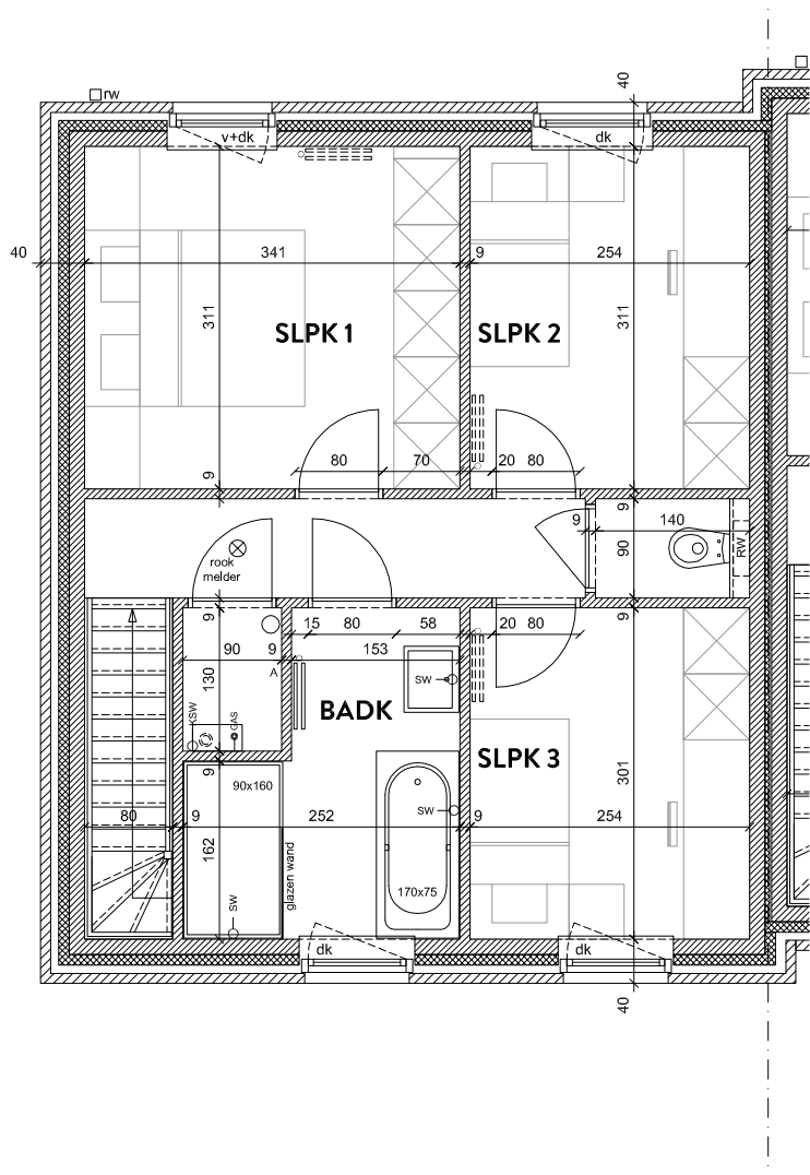
VERDIEPING OPP. 52,64 M 2
