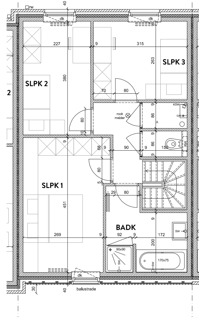
VERDIEPING OPP. 53,27 M 2
