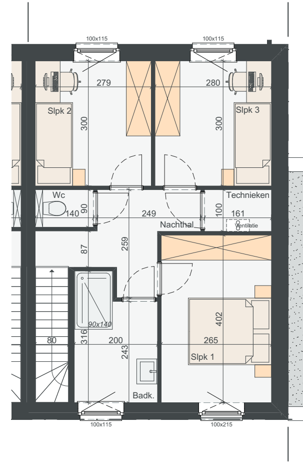
VERDIEPING OPP. ± 56 M 2
