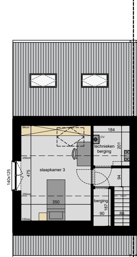
2 DE VERDIEPING OPP. 28,48M 2
