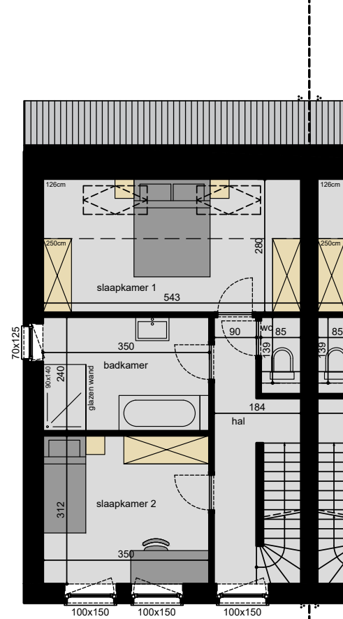
1 STE VERDIEPING OPP. 53,40M 2
