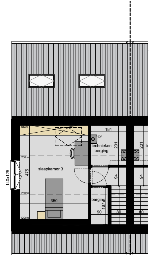
2 DE VERDIEPING OPP. 28,48M 2
