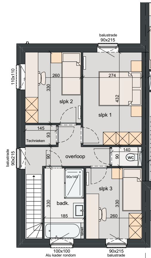
VERDIEPING OPP. 57,42 M 2
