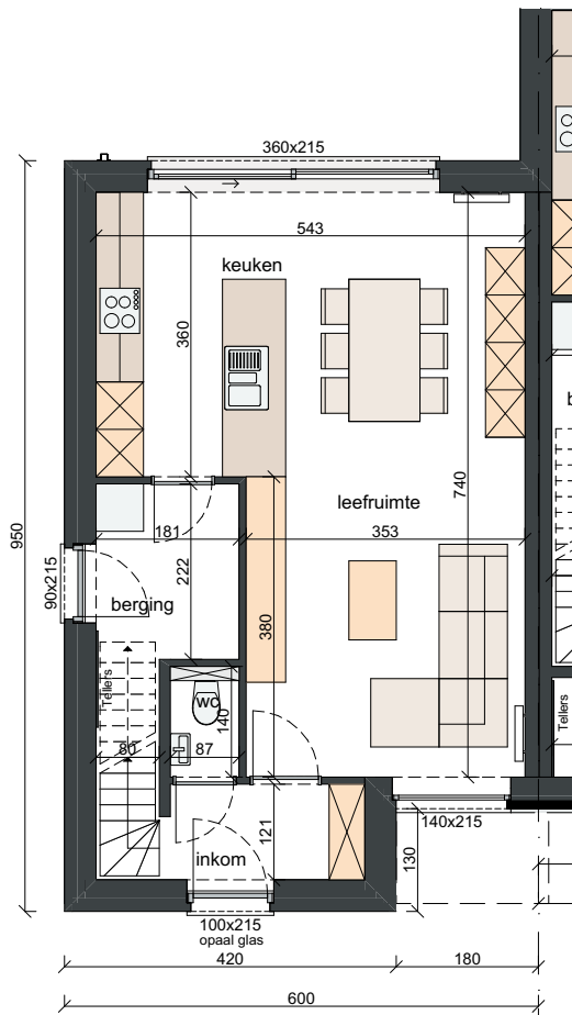
GRONDPLAN OPP. 54,41 M 2
