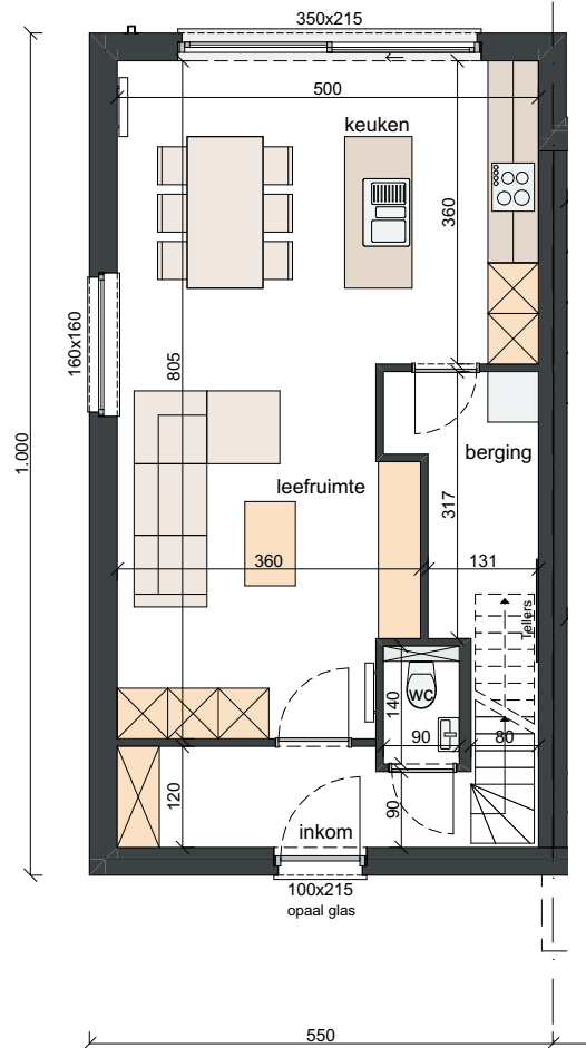
GRONDPLAN OPP. 54,89 M 2
