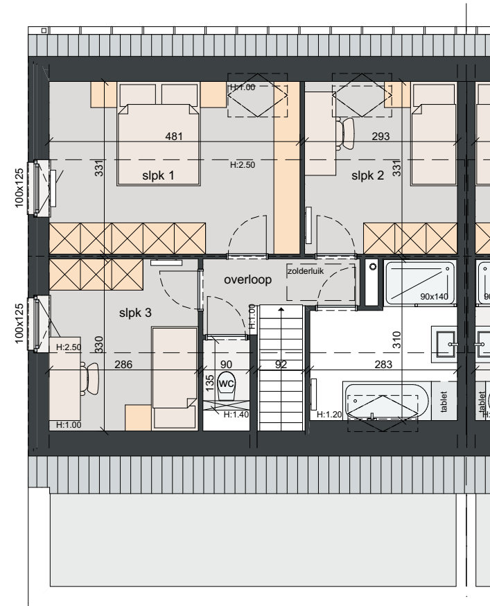
VERDIEPING OPP. 55,04 M 2
