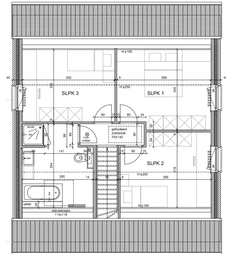
VERDIEPING OPP. 58,78 M 2
