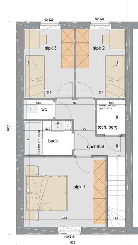
VERDIEPING OPP. 53M 2
