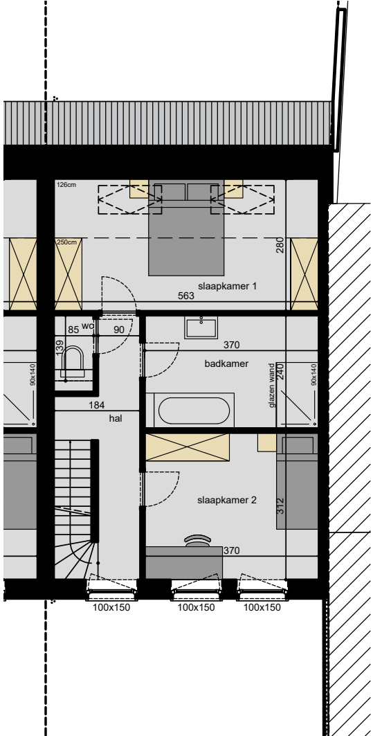
1 STE VERDIEPING OPP. 53,40M 2
