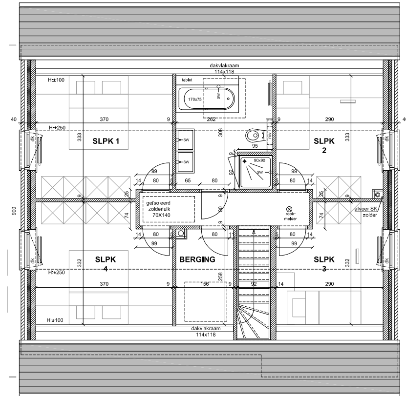
VERDIEPING OPP. 68.75 M 2
